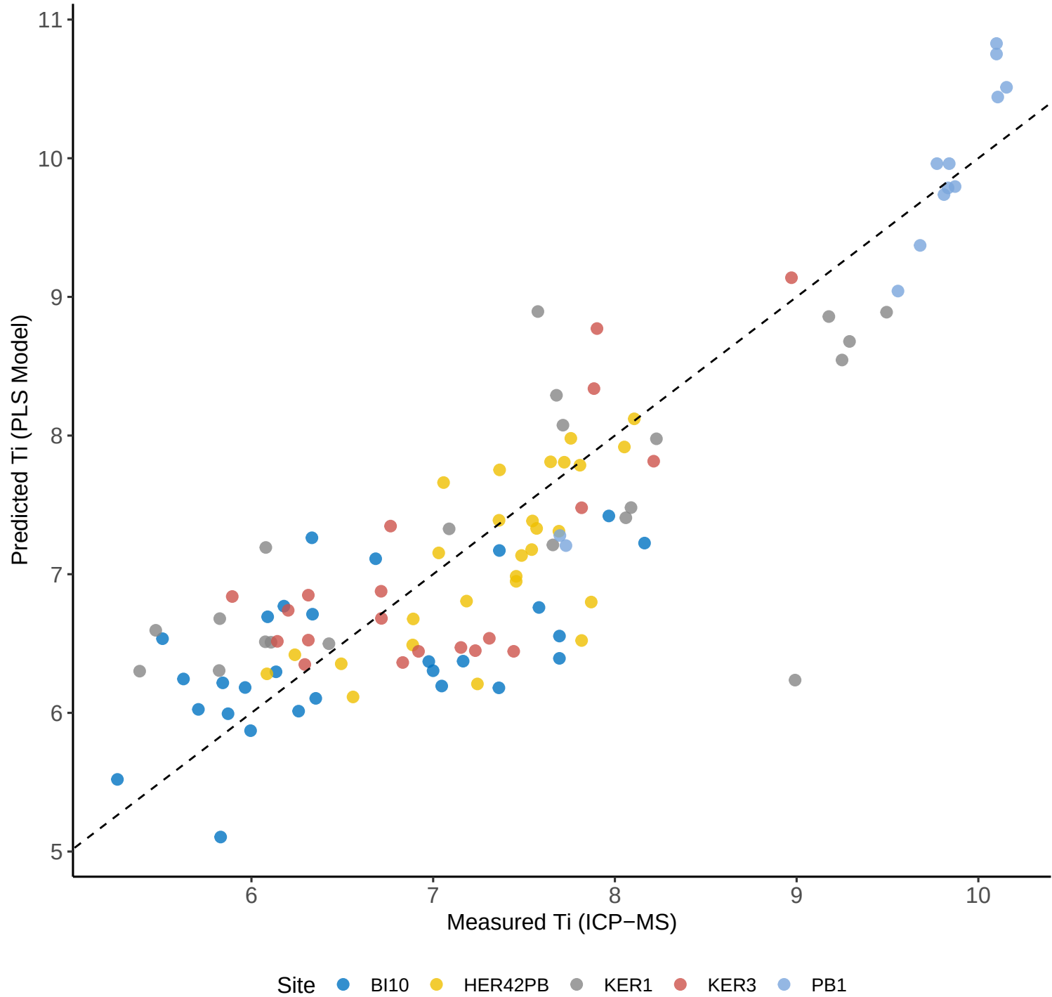
PLS Regression: Measured vs Predicted Titanium (Ti) (30% Test Set)
